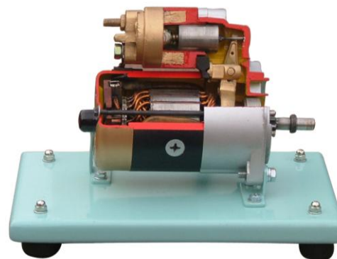
Starter Model Part Number 0204300009
