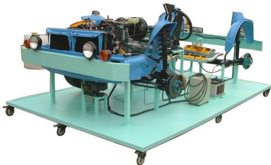
Power Train System Model (Front Drive) Part Number 0204300111
