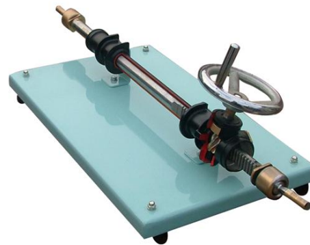
Rack And Pinion Automobile Steering-Gears Model
