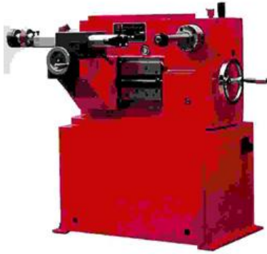
Brake Drumdisc Cutting Machine Part Number 0204100500
