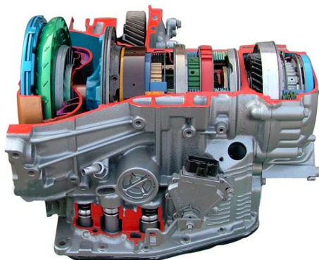
Toyota Front Drive Automatic Transmission Cutaway Model A Part Number 0204300104
