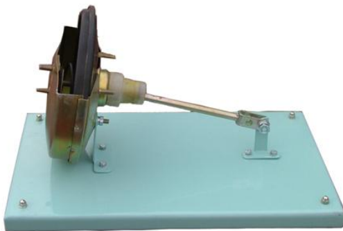
Vacuum Booster Assembly Model Part Number 0204300204
