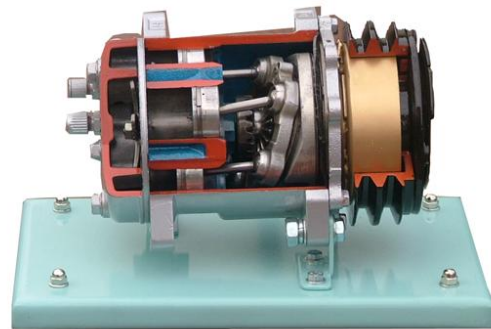
Compressor Model 2 Part Number 0204300203
