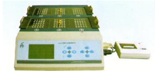
Darkness Avoidance Instrument For Mice Part Number 0202061300
