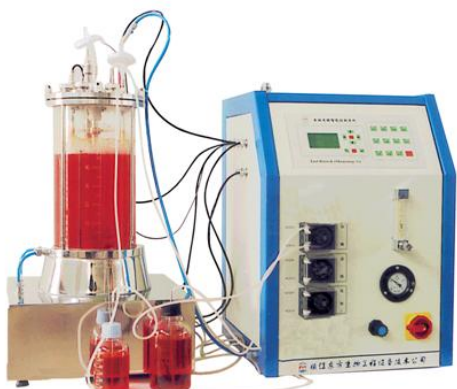
Mechanical Stirred Glass Fermenter Part Number 0202022100
