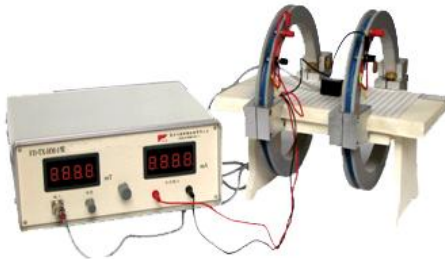
NEW-TYPE MAGNETIC FIELD MEASURING INSTRUMENT WITH CIRCULAR COIL AND HELMHOLTZ COIL
